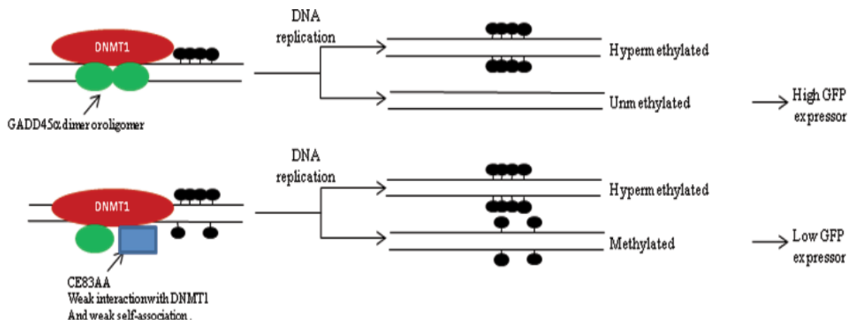
Fig. 6. A model for DNMT1/GADD45 \alpha interplay during HR repair. The figure illustrates the possible interplay between DNMT1 and GADD45 \alpha during HR leading to silencing, low expression, or high expression of HR DNA segments. Filled rollipop represent methylated CpGs induced by HR. In this model, GADD45 \alpha modulates DNMT1 activity at HR site. Depends on availability of GADD45 \alpha , HR DNA segments could be hyper- or hypomethylated.
