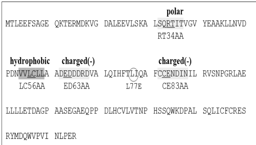
Fig. 3. The position of point mutation in GADD45 \alpha point mutants. The GADD45 \alpha protein is a small, acidic protein of 165 amino acid residues. It does not have any distinct motif or domain. To determine the region of GADD45 \alpha involved in interaction with DNMT1, we systematically changed two consecutive amino acids, which reside in clustered charged, polar, or hydrophobic regions. We generate four point mutants, RT34AD (R34A, T35D), LC56AA (L56A, C57A), ED63AA (E63A, D64A) and CE83AA (C83A, E84A). Two consecutive amino acid residues were replaced with two alanine residues.
