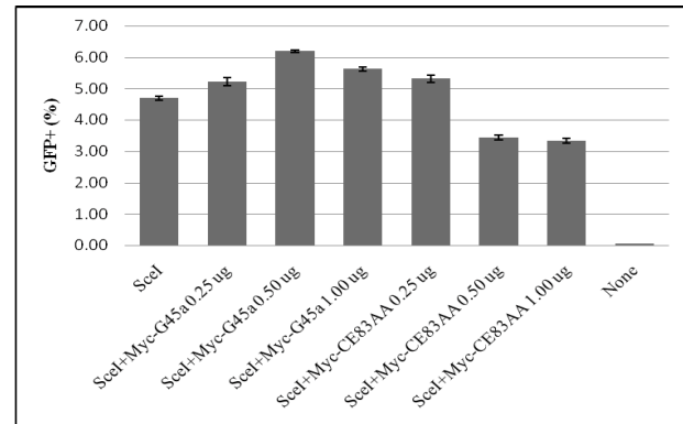
Fig. 5. The stimulation of recombinant GFP gene expression by GADD45 \alpha . HeLa-DRGFP cells were transfected with 2 mg of SceI plasmid and different amount of Myc-GADD45 \alpha or Myc-GADD45 \alpha CE83AA. After 7 days, GFP + cells were analyzed by FACS. Co-expression of Myc-GADD45 \alpha significantly increased the number of GFP + cells, while CE83AA was ineffective.
