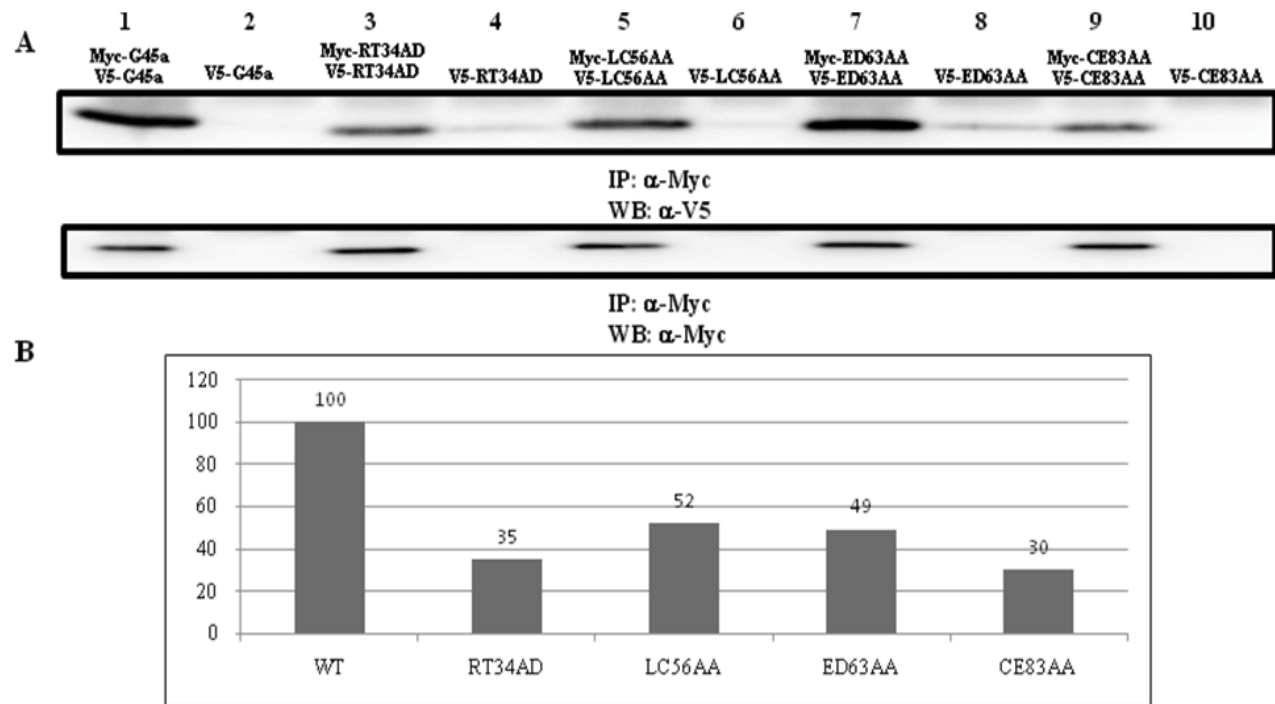
Fig. 4. The self-association of each GADD45 \alpha point mutants. A) Co-immunoprecipitation of each GADD45 \alpha point mutants. B) Quantification of band intensity. The amount of co-immunoprecipitated each GADD45 \alpha point mutants was normalized by the amount of immunoprecipitated each GADD45 \alpha point mutants and the relative level of each band against wild type was plotted.
