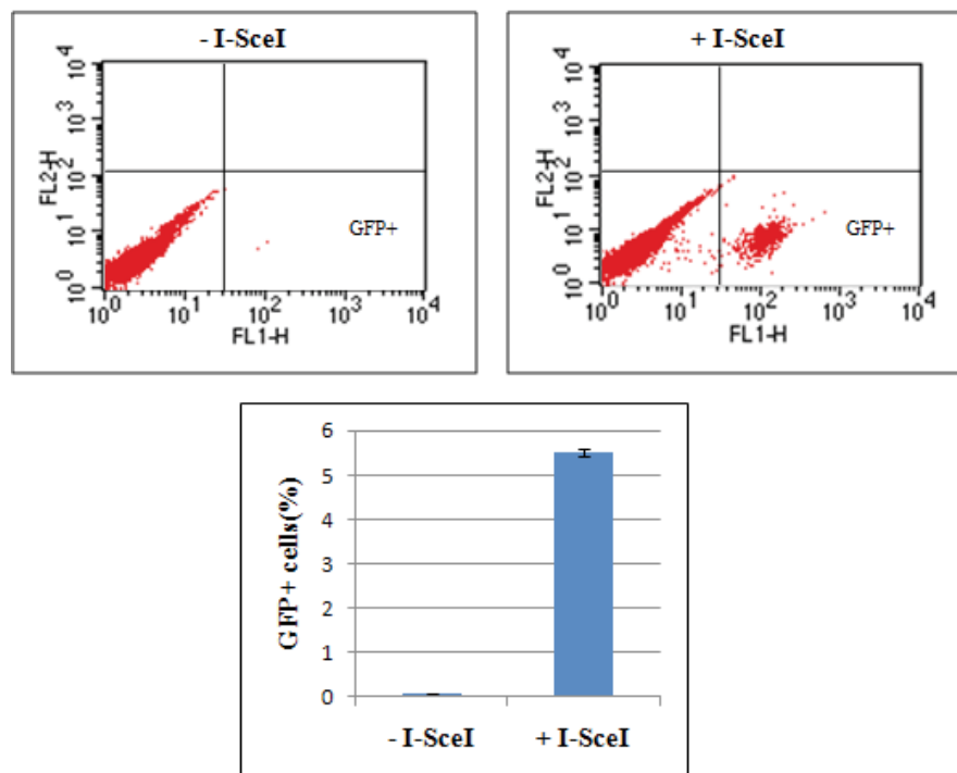
Fig. 2. Recombination assay. About 5.5% of cells expressed GFP and the GFP expression was observed in cells transfected with I-SceI plasmid. Control cells, which were not transfected with I-SceI plasmid showed background level fluorescence revealing that HR was induced by DSB.
