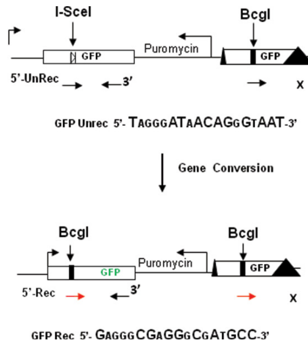
Fig. 1. Formation of a functional GFP gene by recombination initiated at a specific DSB [7].
